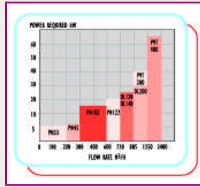
PN - Rotary Vane Vacuum
